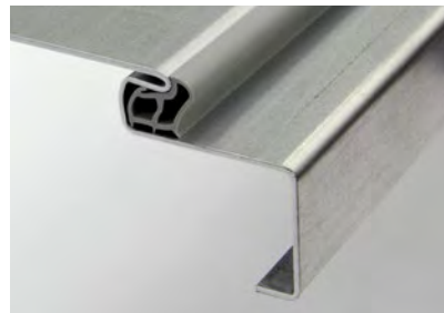
Precise flange dimensions, angles and straightness of the profiles.
